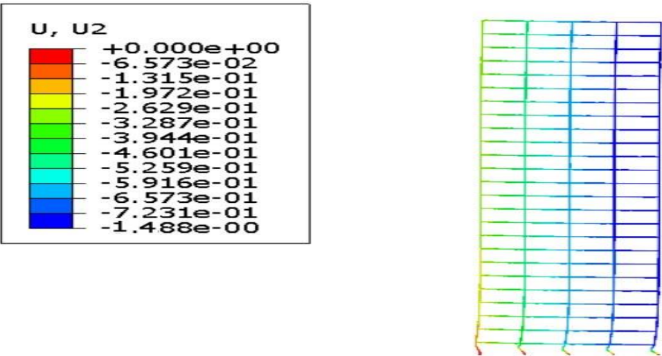
Figure 20: The highest displacement in thermal analysis in model number 18 (simple frame, 25-floor model, fire location next to the first floor of the structure)
