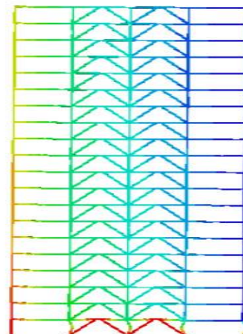
Figure 16: The largest displacement in thermal analysis in model number 14 (frame with divergent brace, 20-floor model, fire location next to the first floor of the structure)
