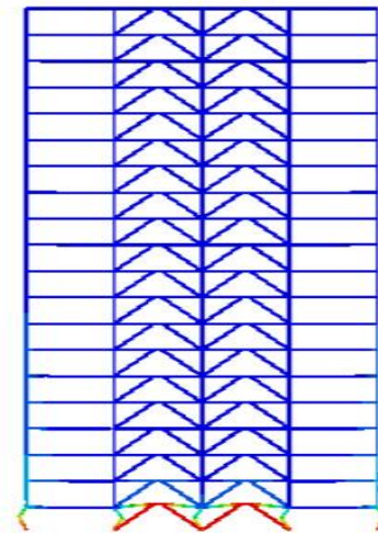
Figure 15: The highest displacement in thermal analysis in model number 13 (frame with diverging brace, 20-floor model, fire place in the middle of the first floor of the structure)
