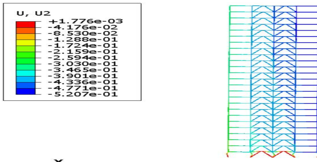
Figure 24: The highest displacement in thermal analysis in model number 22 (frame with divergent brace, 25-floor model, fire location next to the first floor of the structure)
