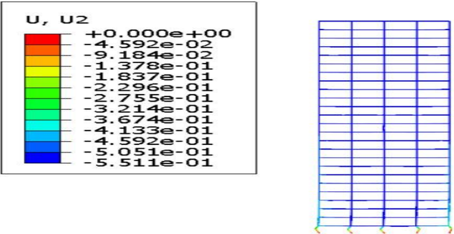
Figure 21 : The highest displacement in thermal analysis in model number 19 (simple frame, 25-floor model, fire place in the middle of the middle floor of the structure)
