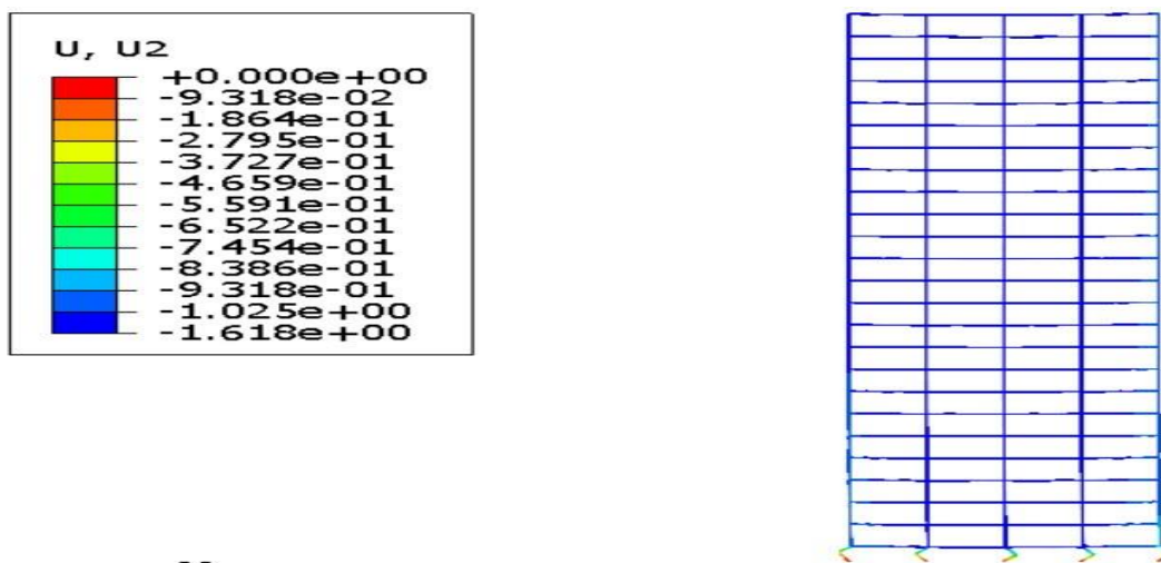
Figure 19: The highest displacement in thermal analysis is in model number 17 (simple frame, 25-floor model, fire place in the middle of the first floor of the structure).
