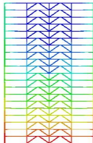
Figure 16: The largest displacement in thermal analysis in model number 14 (frame with divergent brace, 20-floor model, fire location next to the first floor of the structure)
