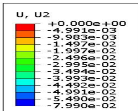
Figure 16: The largest displacement in thermal analysis in model number 14 (frame with divergent brace, 20-floor model, fire location next to the first floor of the structure)
