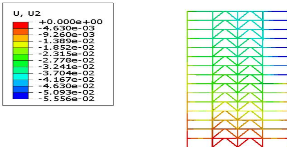
Figure 9: The highest displacement in thermal analysis in model number 7 (frame with divergent brace, 15-floor model, fire location in the middle of the middle floor of the structure)
