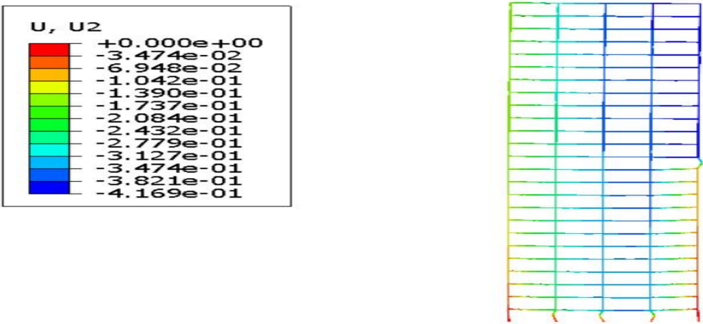
Figure 21 : The highest displacement in thermal analysis in model number 19 (simple frame, 25-floor model, fire place in the middle of the middle floor of the structure)
