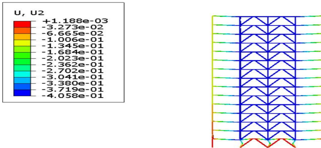
Figure 7: The highest displacement in thermal analysis is in model number 5 (frame with divergent brace, 15-floor model, fire place in the middle of the first floor of the structure)
